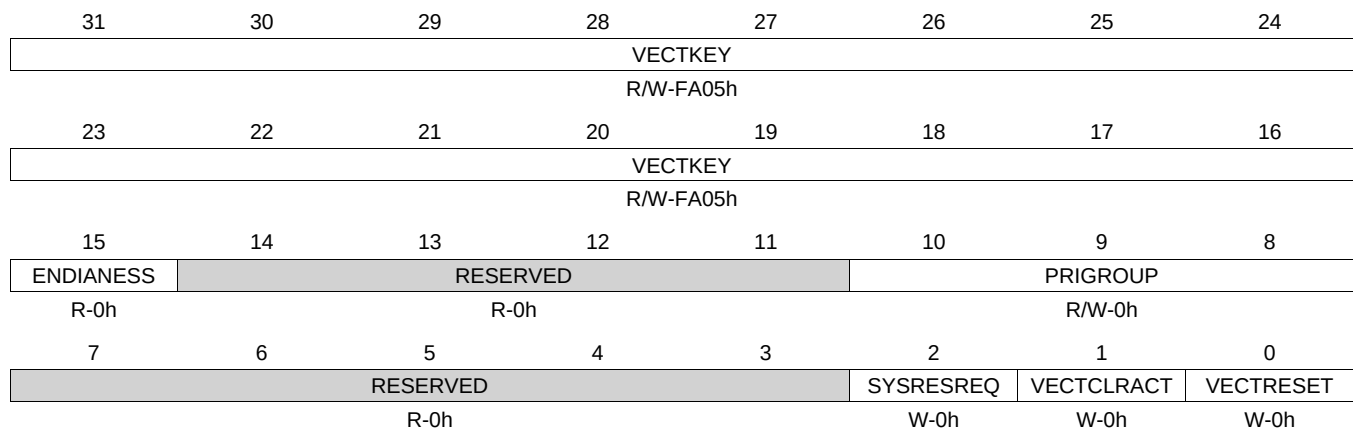
Figure 3-14. APINT Register
