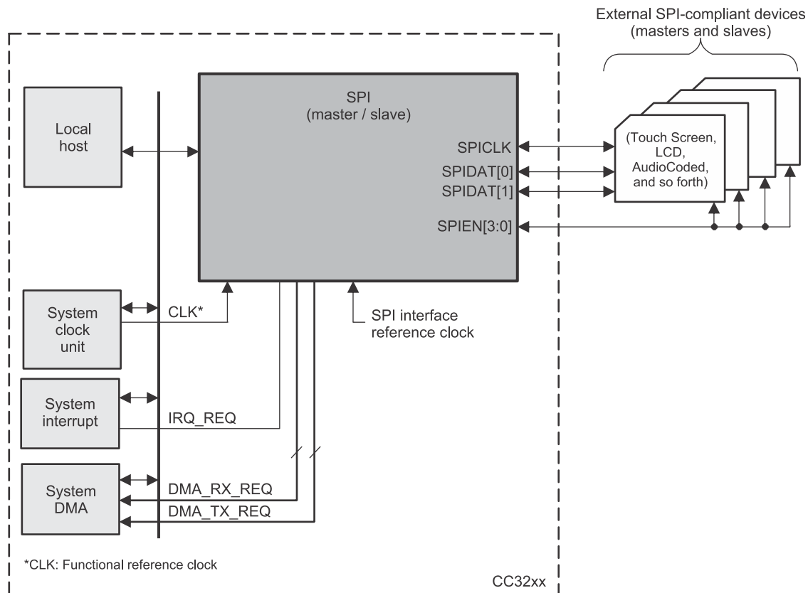
Figure 8-1. SPI Block Diagram
