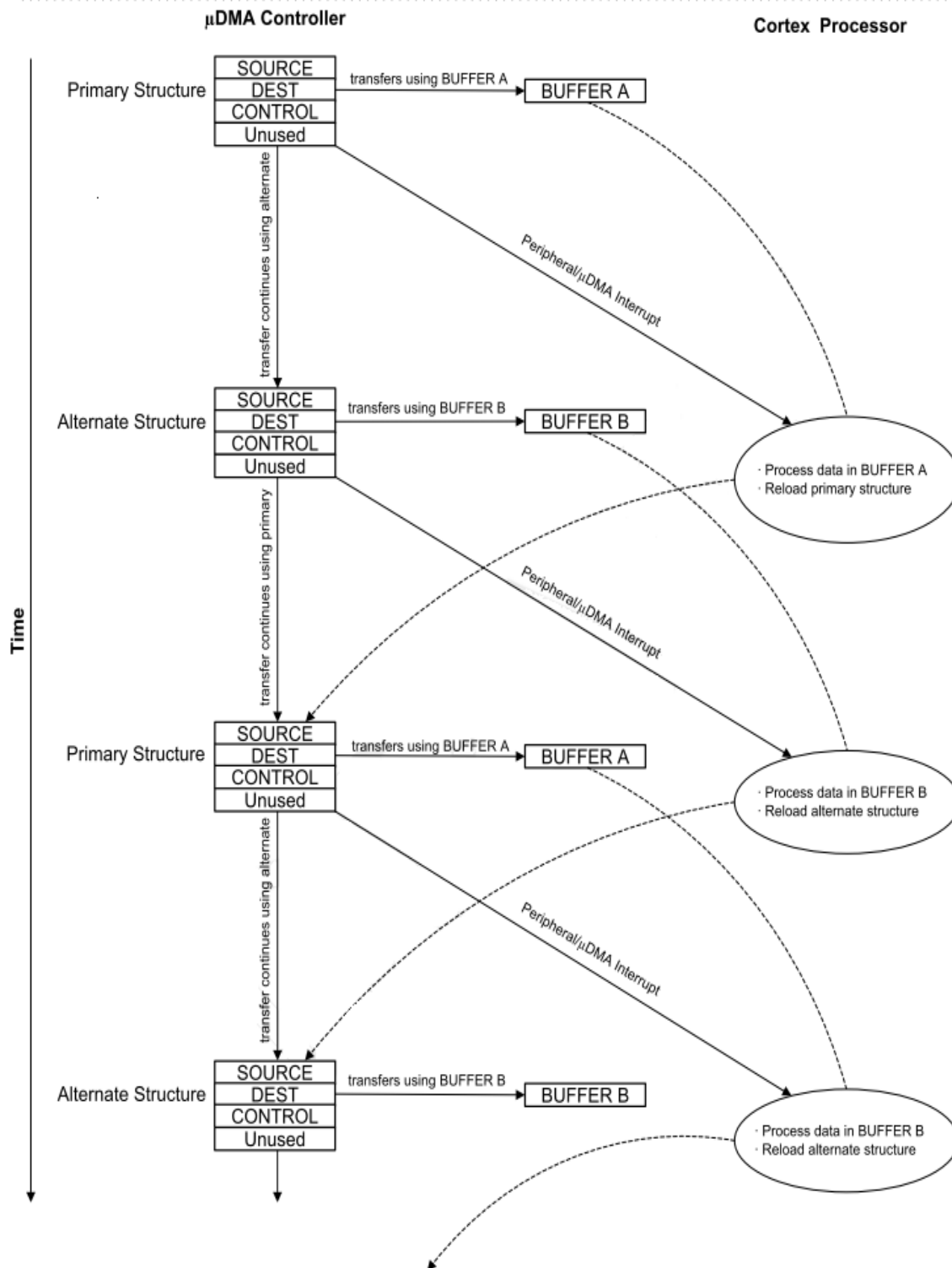
Figure 4-2. Ping-Pong Mode
