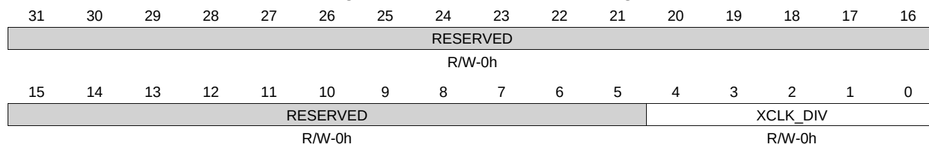
Figure 14-15. CC_CTRL_XCLK Register
