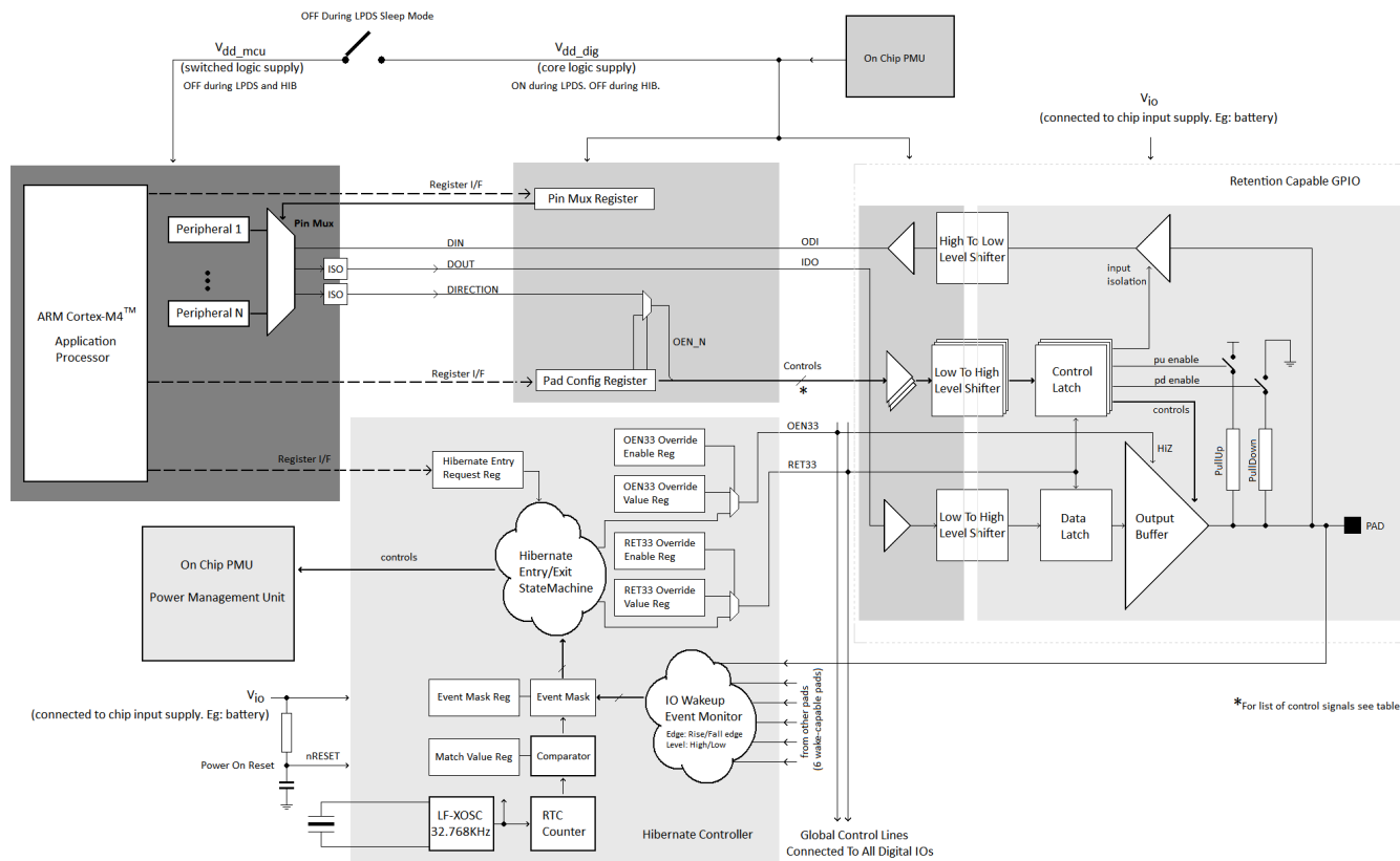
Figure 16-3. I/O Pad Data and Control Path Architecture in CC3200
