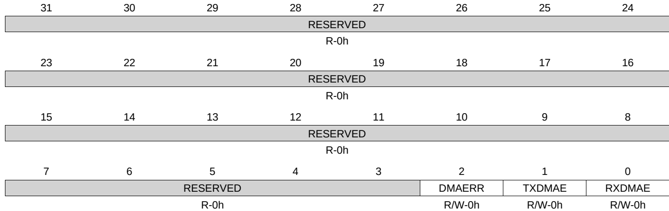
Figure 6-14. UARTDMACTL Register
