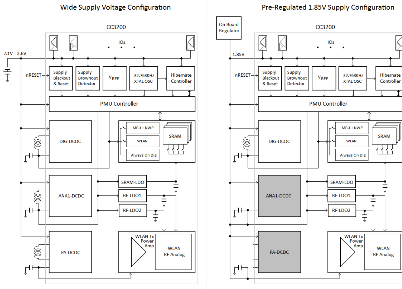
Figure 15-1. Power Management Unit Supports Two Supply Configurations
