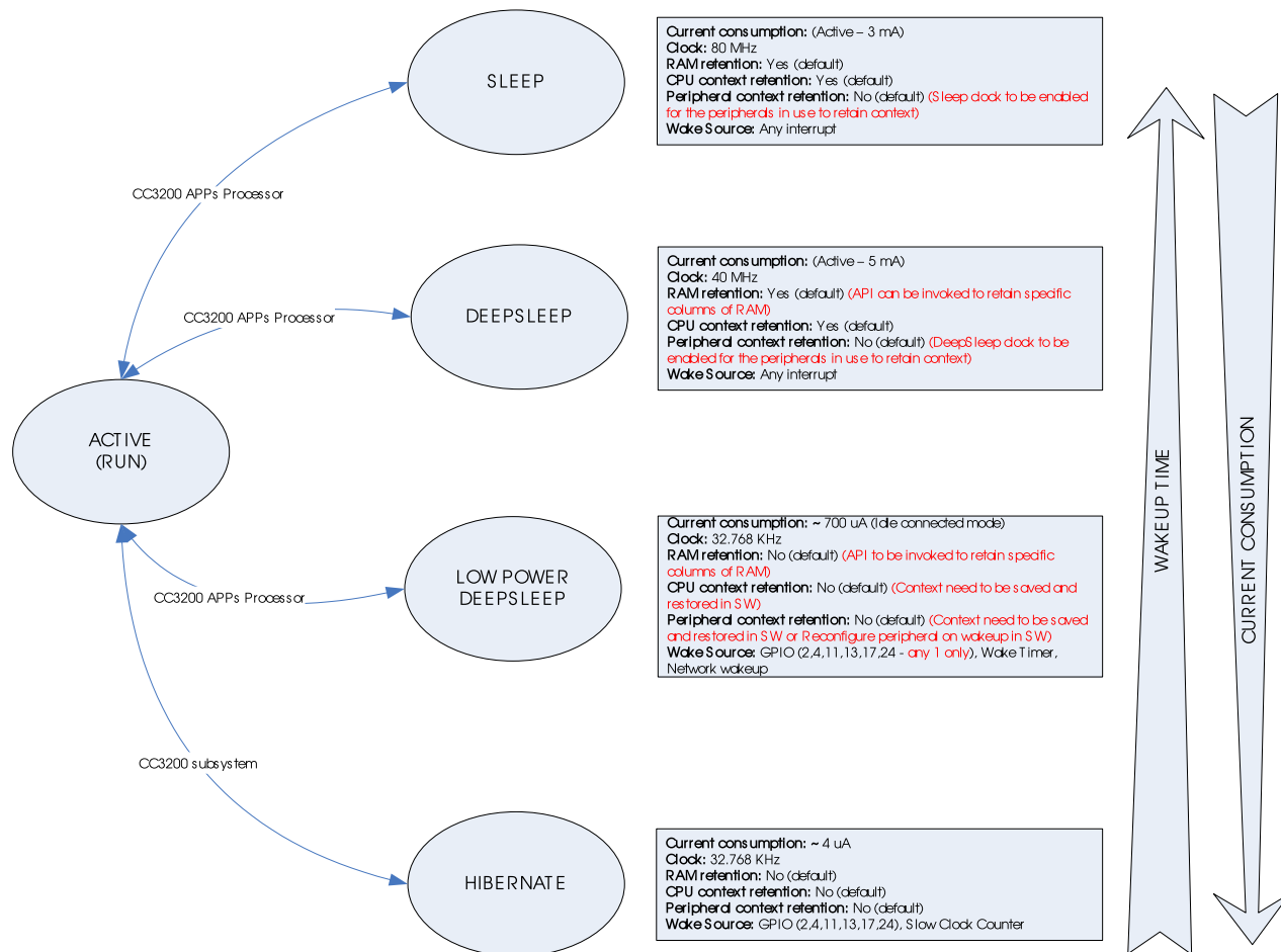
Figure 15-2. Sleep Modes
