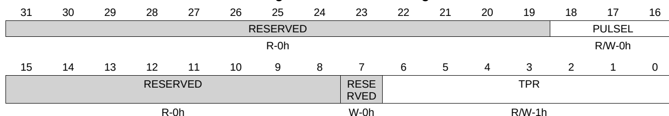
Figure 7-17. I2CMTPR Register
