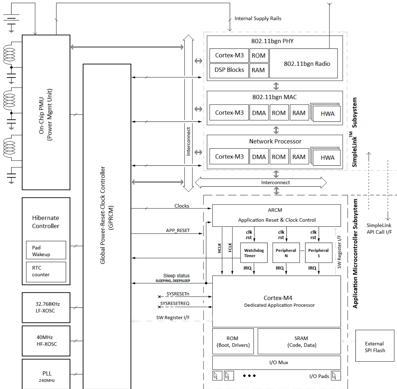
Figure 15-3. Power Management Control Architecture in CC3200
