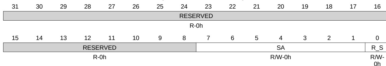
Figure 7-14. I2CMSA Register
