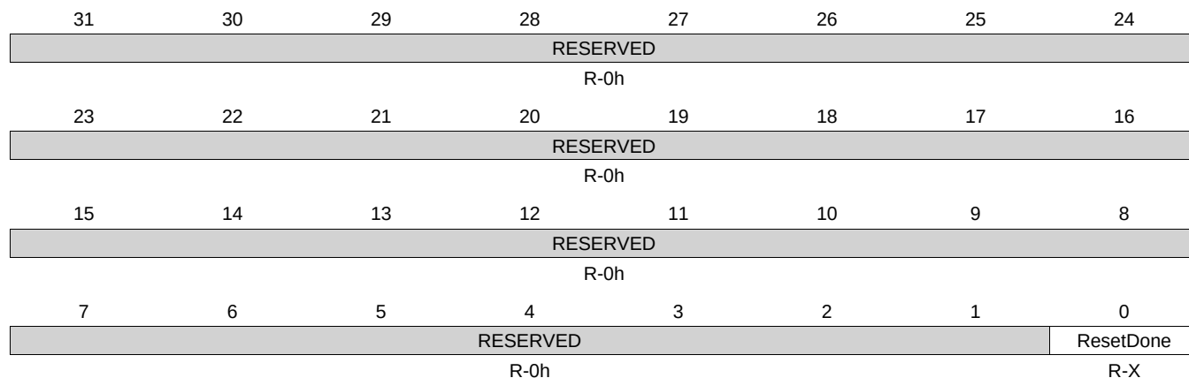
Figure 14-10. CC_SYSSTATUS Register
