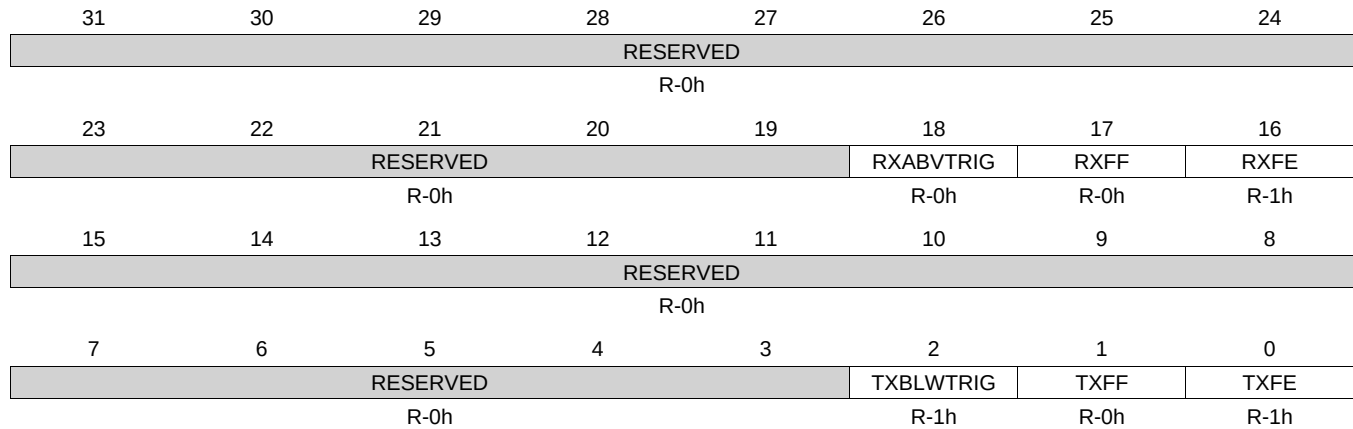
Figure 7-38. I2CFIFOSTATUS Register
