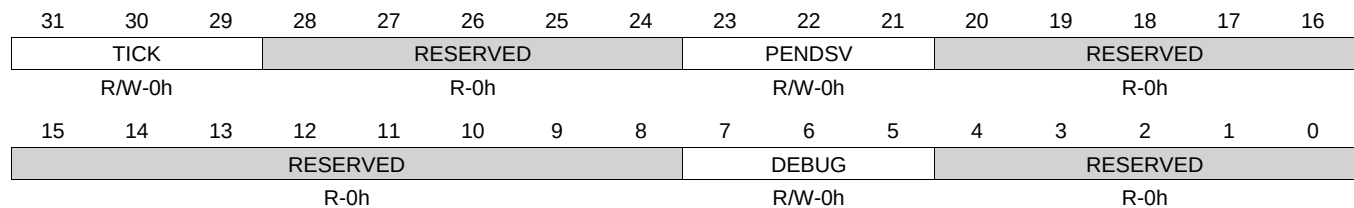
Figure 3-19. SYSPRI3 Register
