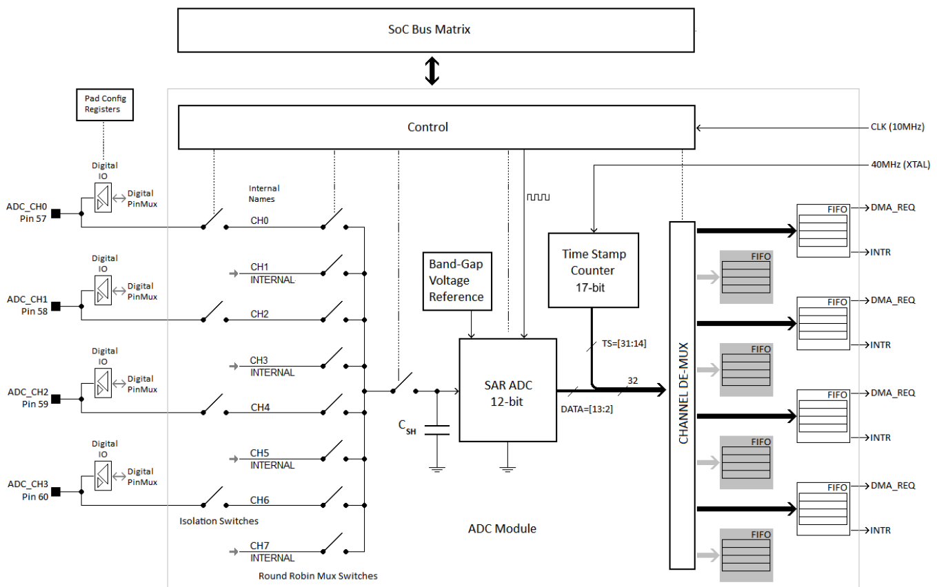
Figure 13-1. Architecture of the ADC Module in CC3200
