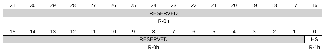
Figure 7-39. I2CPP Register
