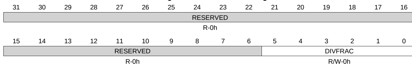
Figure 6-6. UARTFBRD Register
