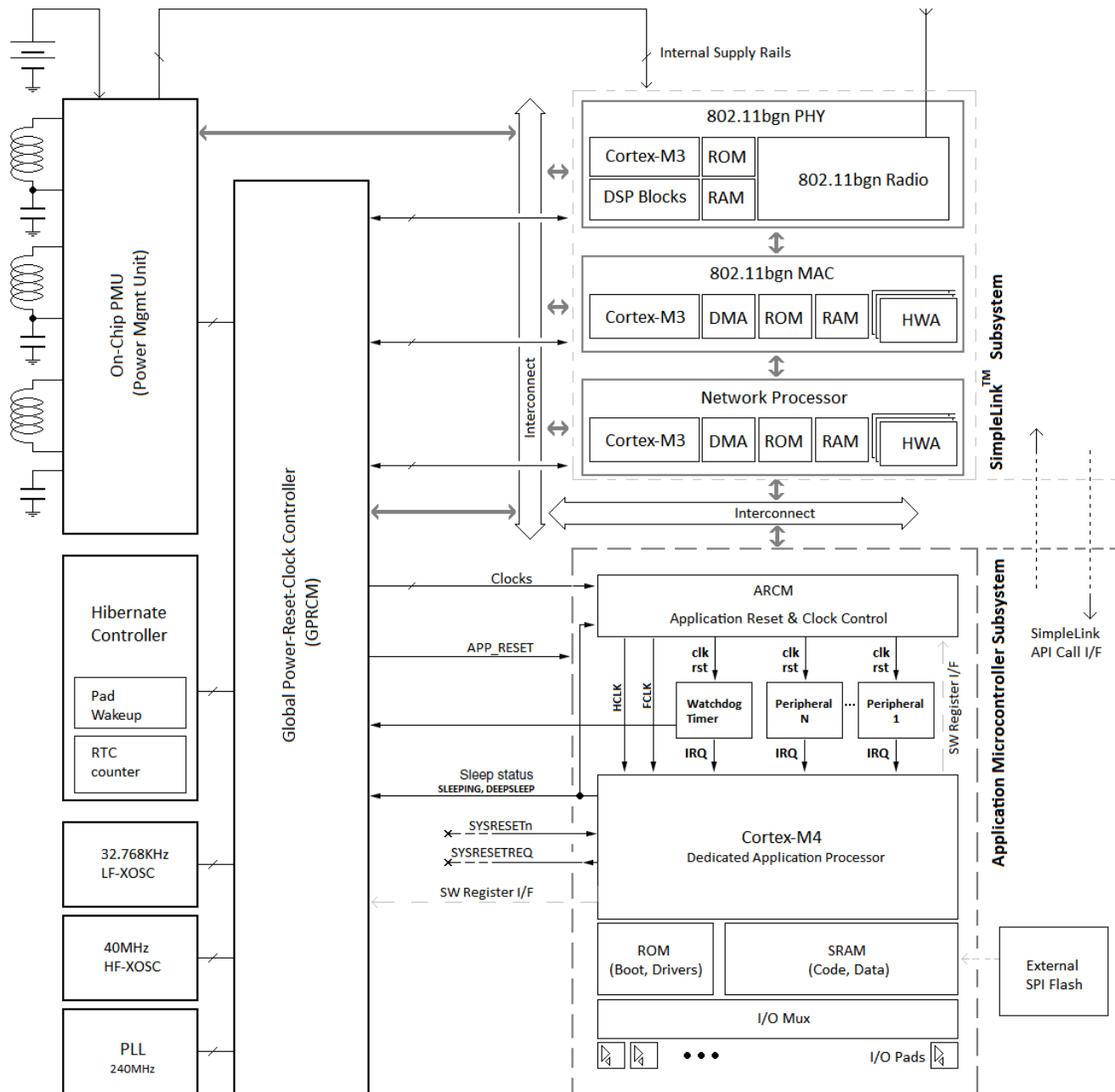
Figure 2-7. Power Management Architecture in CC3200 SoC
