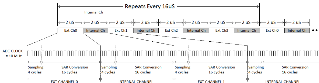
Figure 13-2. Operation of the ADC
